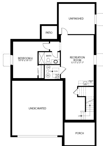
FINISHED FULL BASEMENT-1
