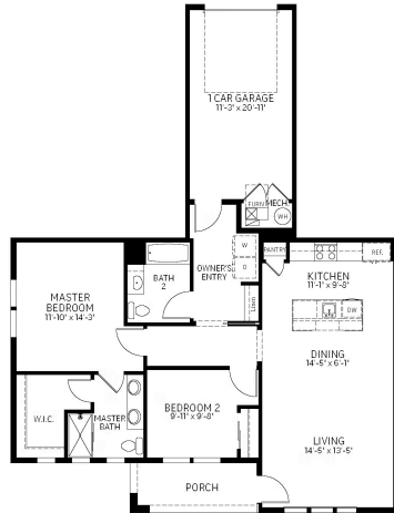
FLOOR PLAN
