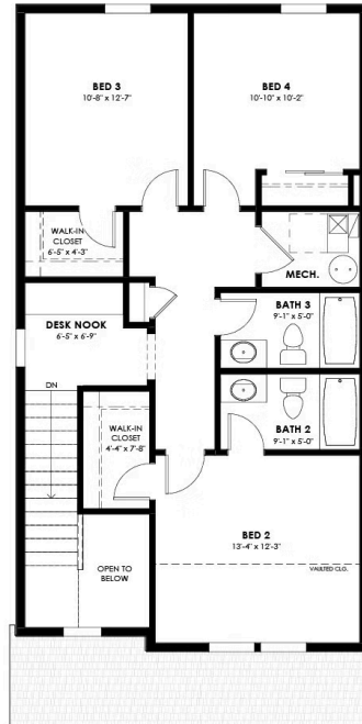
PAIRED HOMES WILLOW UNIT "A" - SECOND LEVEL
